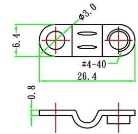
CABLE CLAMP: STEEL IN NICKEL PLATED (2 pcs)
