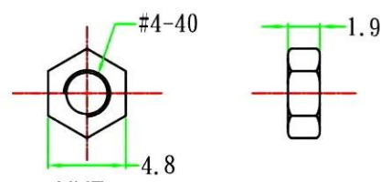
NUT: STEEL IN NICKEL PLATED (2 pcs)
