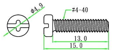
FIXED SCREW: STEEL IN NICKEL PLATED PHILLIPS HEAD (2 pcs)
