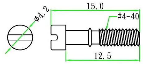
SCREW: STEEL IN NICKEL PLATED (2 pcs) SLOTTED HEAD
