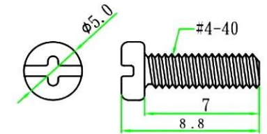
SCREW: STEEL IN NICKEL PLATED 2(pcs)
