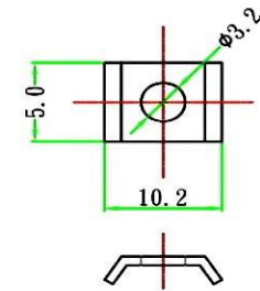
WASHER: STEEL IN NICKEL PLATED (2 pcs)
