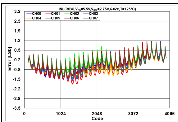
FIGURE 2-112: INL Error vs. DAC Code, T = +125^\circ\text{C} , V_{DD} = 5.5\text{V} .
