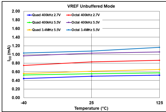
FIGURE 2-7: Average Device Supply Current vs. F_{SCL} Frequency, Voltage and Temperature - Active Interface, V_{REF} Unbuffered Mode). VRnB:VRnA = 10 ( V_{REF} Unbuffered Mode).
