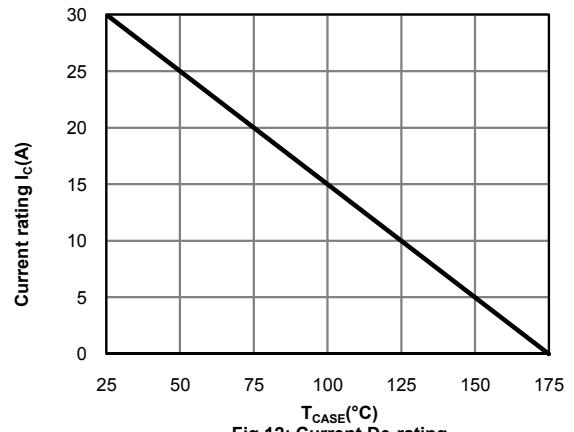
Fig 12: Current De-rating
