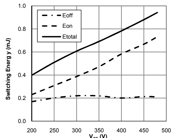
Figure 20: Switching Loss vs. V_{CE} ( T_j=175^\circ\text{C}, V_{GE}=15\text{V}, I_c=15\text{A}, R_g=20\Omega )
