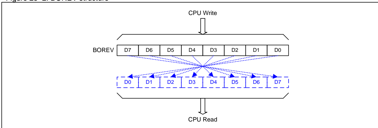
Figure 25–2. BOREV structure
