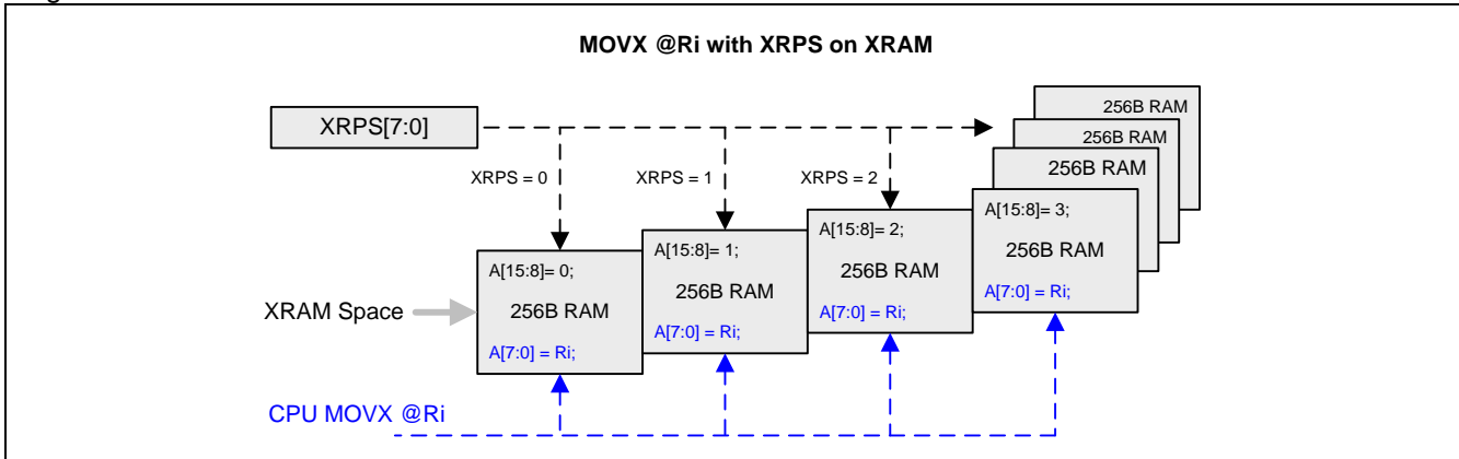
Figure 7–2. XRPS Structure
