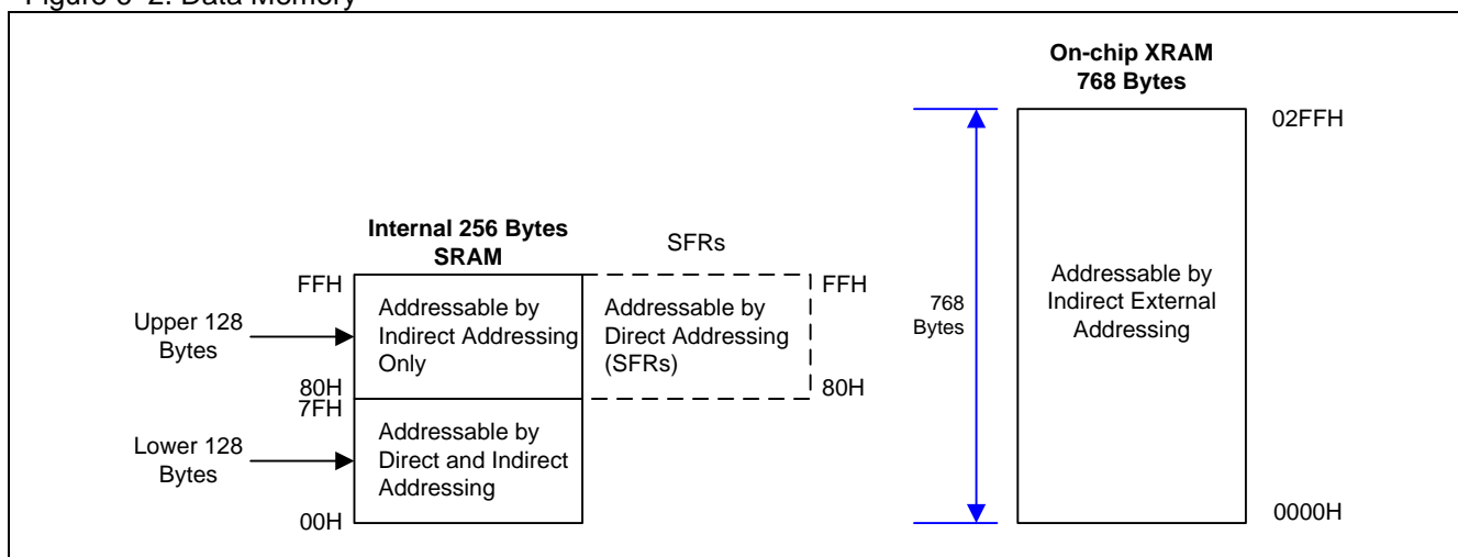
Figure 6–2. Data Memory
