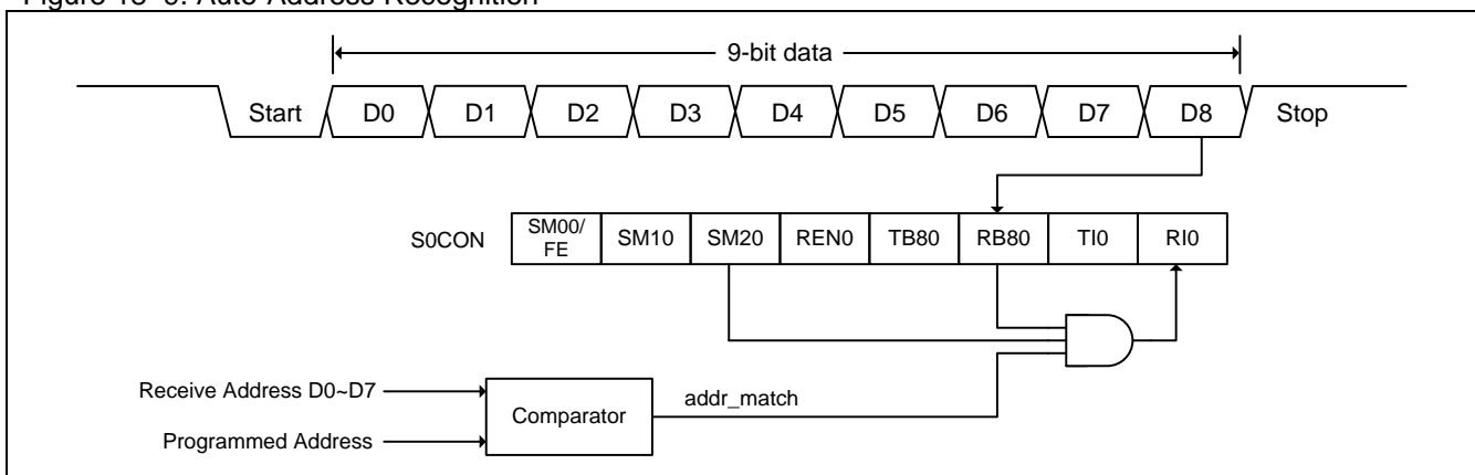
Figure 18–9. Auto-Address Recognition
