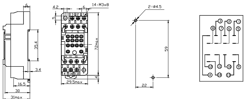
18FF-4C-D2 Dimension PCB layout Inter Connection
