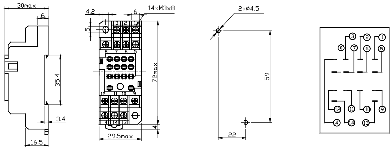
18FF-4C-D2 Dimension PCB layout Inter Connection
