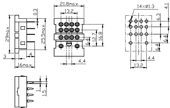
18FF-4C-D1 Dimension PCB layout Inter Connection
