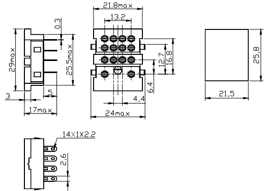
18FF-4C-A2 Dimension Mounting Holes
