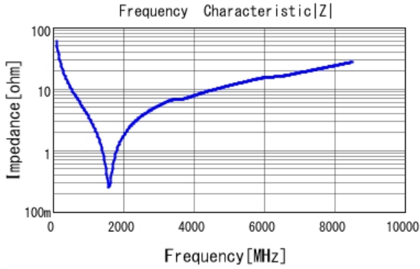
■ GRM1555C1H270JA01 |Z| DC0V, 25degC
